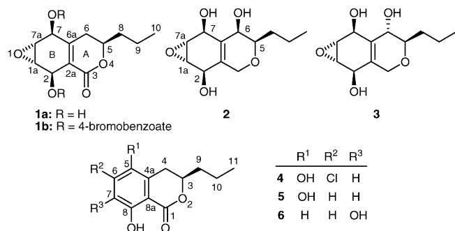
Figure 1. Structures of compounds 1a , 2–6 isolated from Phomopsis sp.
