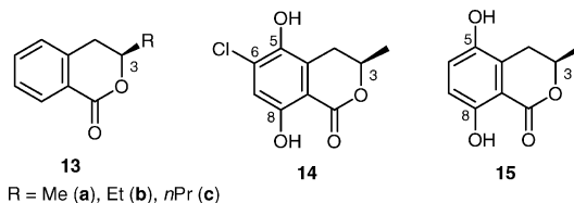
Figure 9. Compounds considered in the calculations.
