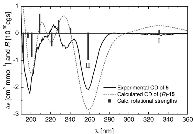
Figure 8. Measured (MeCN) CD spectrum of 5 (solid line) compared with TDDFT-calculated CD of ( R )- 15 (grey dotted line, Boltzmann-weighted average over 4 DFT minima). Vertical bars represent computed rotational strengths R .
