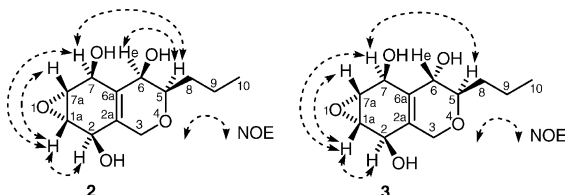
Figure 6. Selected NOE correlations for cycloepoxytriol A ( 2 ) and cycloepoxytriol B ( 3 ).
