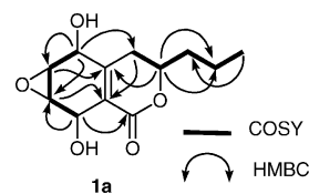
Figure 3. Summary of ^1\text{H} - ^1\text{H} COSY and ^1\text{H} - ^{13}\text{C} HMBC for 1a .
