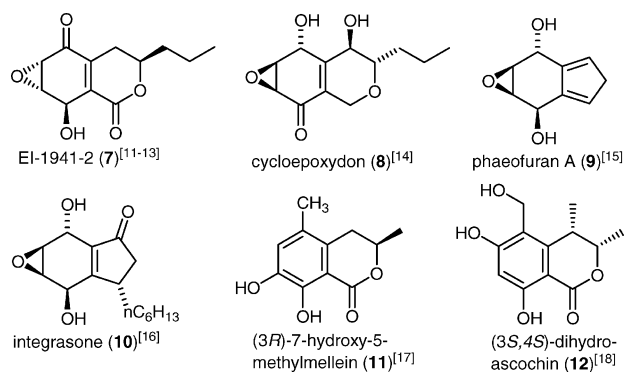
Figure 2. Structures of related hydroxycyclohexene epoxides ( 7–10 ) and dihydroisocoumarins ( 11 , 12 ) from the literature.
