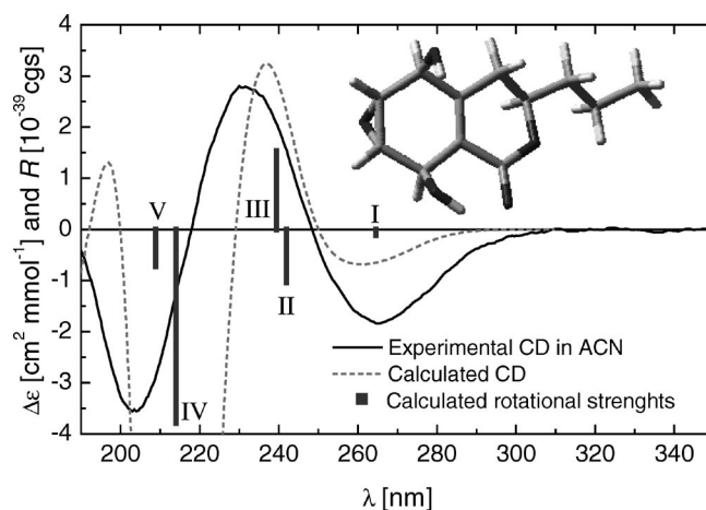
Figure 5. Measured (MeCN, solid line) and TDB3LYP/TZVP-calculated (dotted line) CD spectra of (1 a S,2 R ,5 R ,7 S ,7 a R)- 1a by using the lowest-energy DFT structure drawn in the inset. Vertical bars represent computed rotational strengths R .
