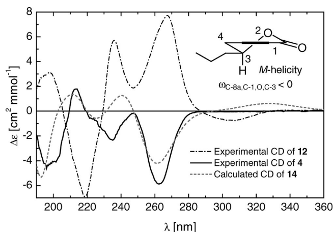
Figure 7. Measured (MeCN) CD spectrum of 4 (solid line) compared with TDDFT-calculated CD of ( R )- 14 (grey dotted line, Boltzmann-weighted average over 2 DFT minima) and experimental CD of 12 (dashed-dotted line). Inset: ( M ) helicity of the dihydroisocoumarin heteroring with equatorial C-3 n -propyl group and (3 R ) absolute configuration.
